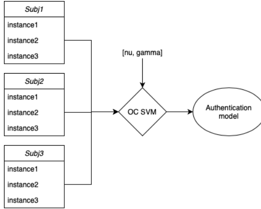
Figure 4.6: Authentication model using OC SVM and common model layout.
