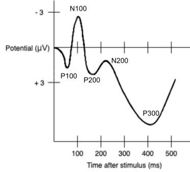
Figure 2.2: ERP waveforms
