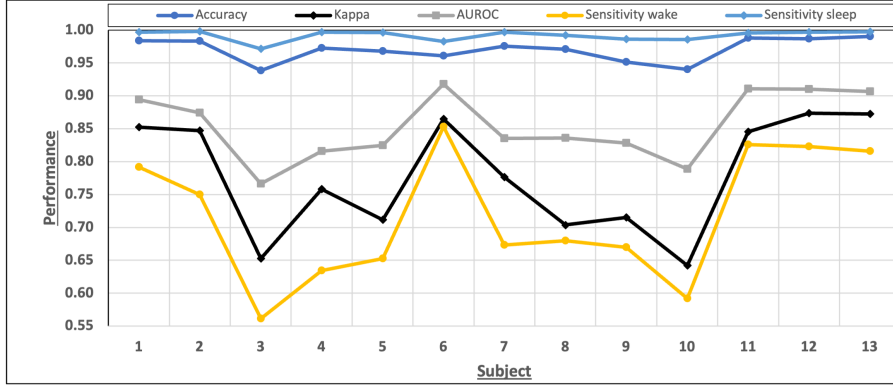
Fig.1: Performance of sleep-wake classification for all subjects using 128 channels.
