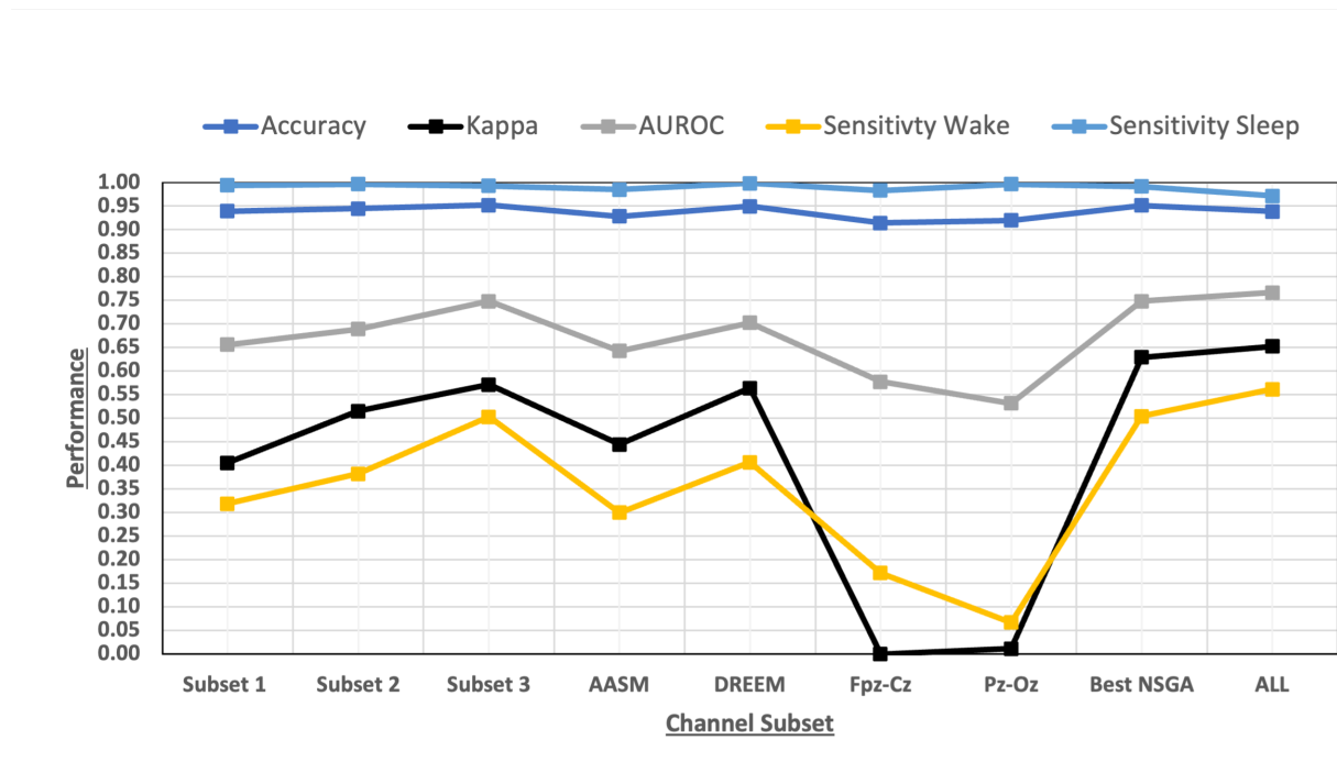
Figure 5.14: Performance of sleep-wake classification for Subject 3 based on different subsets of channels.
