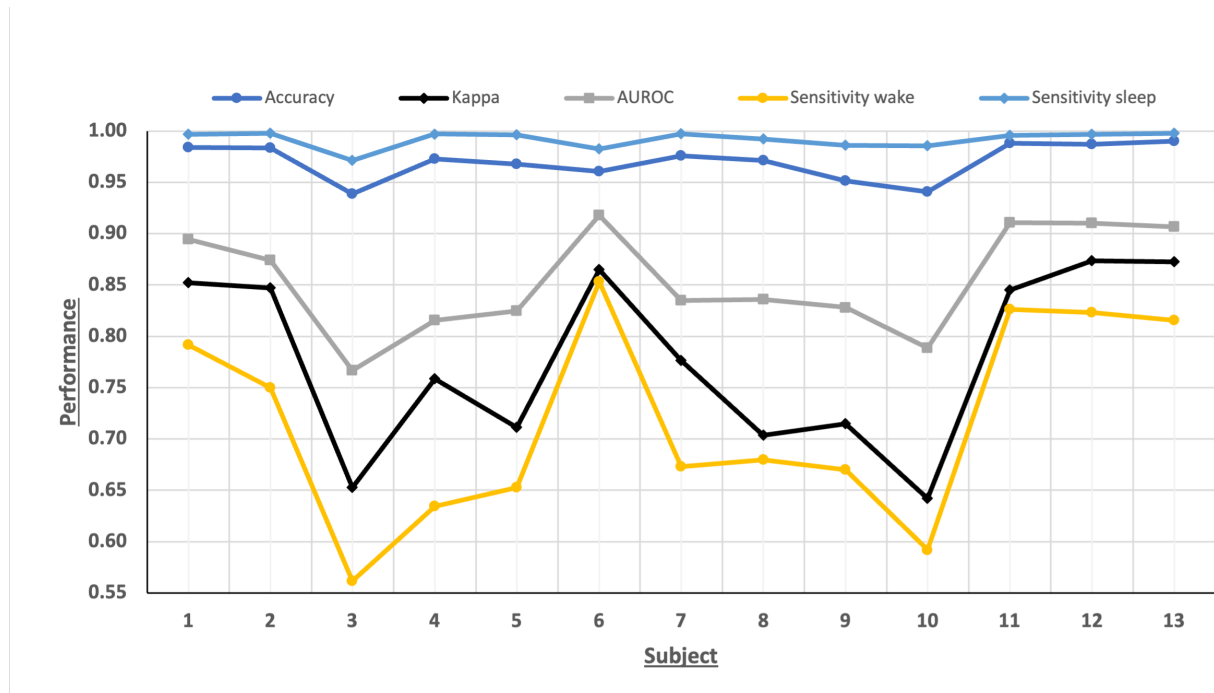
Figure 5.2: Performance of sleep-wake classification for all subjects using 128 high-density EEG channels
