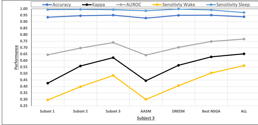
Fig. 3: Performance of sleep-wake classification for subject 3 based on different subsets of channels.
