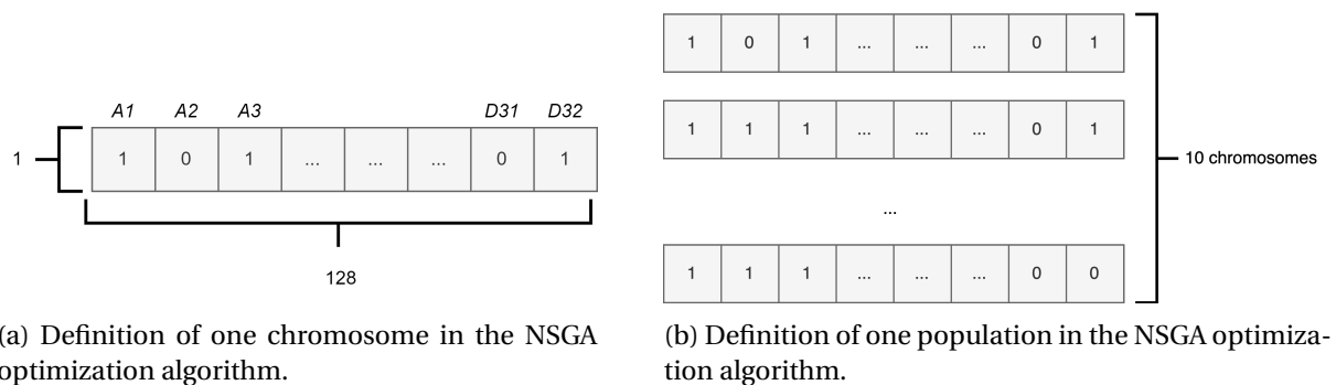
Figure 4.5: Definition of chromosome and population in the NSGA optimization algorithm.
