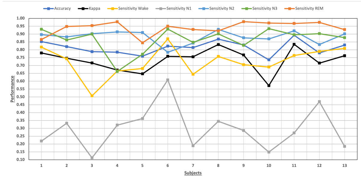
Figure 5.3: Performance of five-class sleep-stage classification for all subjects using all 128 high-density EEG channels
