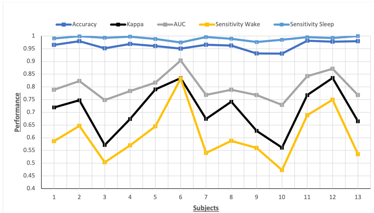
Figure 5.11: Performance of all subjects utilizing NSGA Subset 3.
