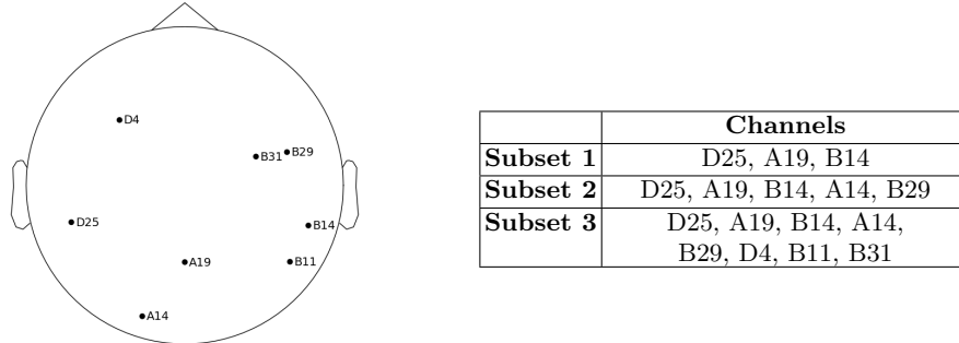
Fig. 6: Positioning and subsets of channels obtained from the NSGA-III analysis.
