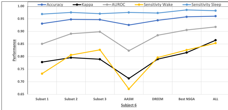
Fig. 4: Performance of sleep-wake classification for subject 6 based on different subsets of channels.
