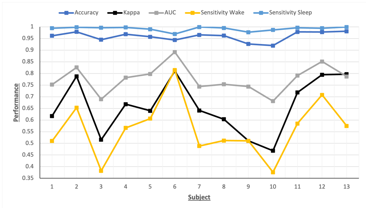
Figure 5.10: Performance of all subjects utilizing NSGA Subset 2.
