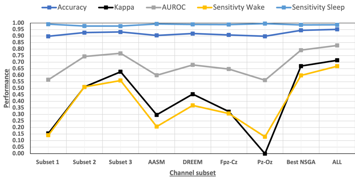
Figure 5.16: Performance of sleep-wake classification for Subject 9 based on different subsets of channels.
