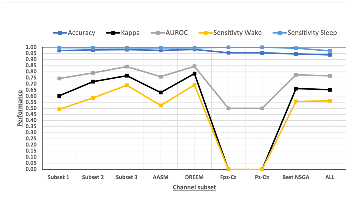
Figure 5.17: Performance of sleep-wake classification for Subject 11 based on different subsets of channels.
