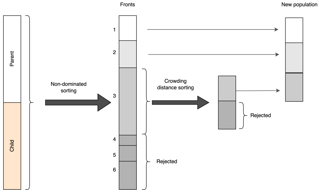
Figure 2.13: Illustration of NSGA procedure. The figure shows how a set of parent and child chromosomes is used to form a new population with non-dominated sorting and crowding distance sorting. Adapted from [56].
