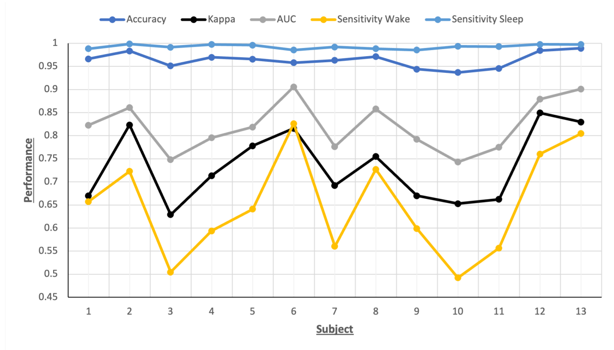
Figure 5.12: Performance of all subjects utilizing its corresponding best subset of channels from the NSGA analysis
