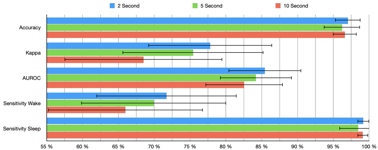
Figure 5.1: Comparison of performance with the use of different segment sizes for each epoch in the dataset. The best-performing segment size is 2 seconds, highlighted in blue.
