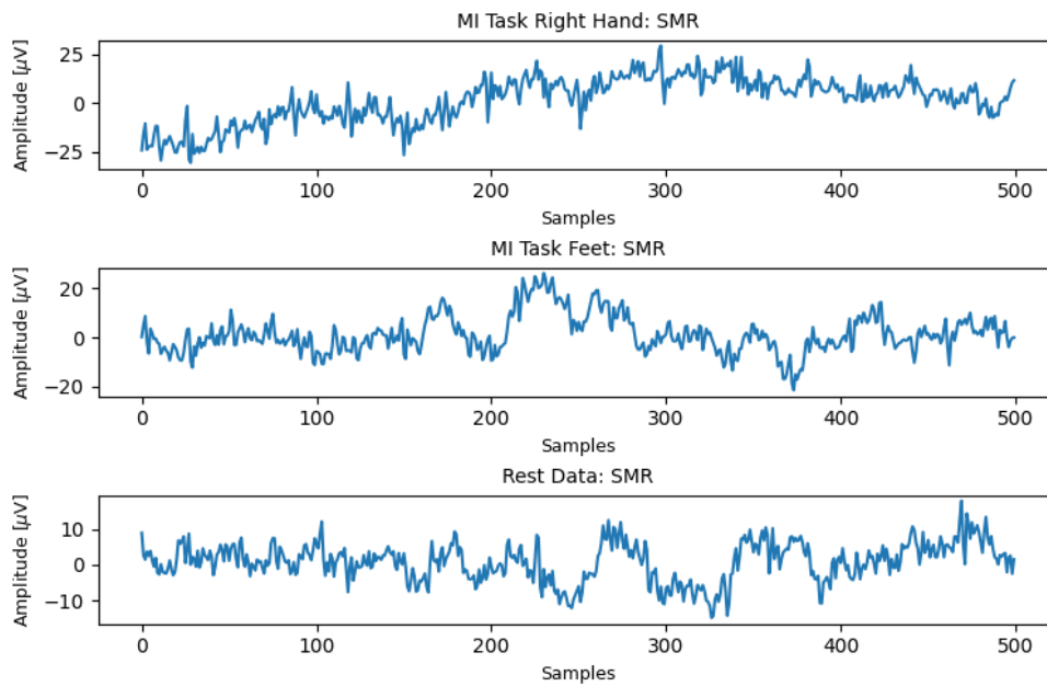
Figure 4.11: The raw EEG signal from dataset SMR with and without MI evoked, respectively. Taken from the first trial of each class in channel C3 for subject S1T.
