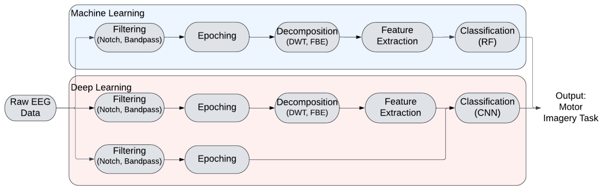
Figure 4.17: The data processing and classification pipeline for the ML and DL algorithms.
