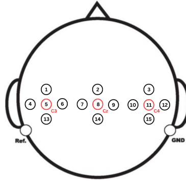
Figure 4.9: Electrode placement for dataset SMR. Based on Laplacian derivations.
