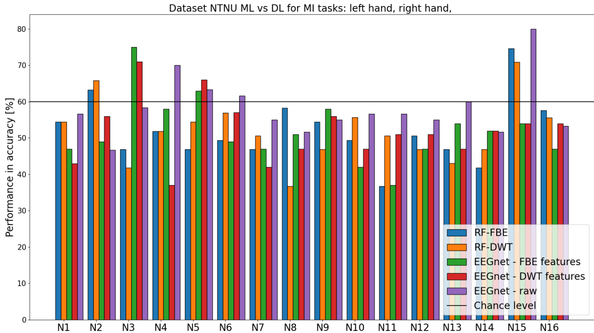
Figure 5.33: Binary classification of left and right-hand for each subject in the NTNU dataset.
