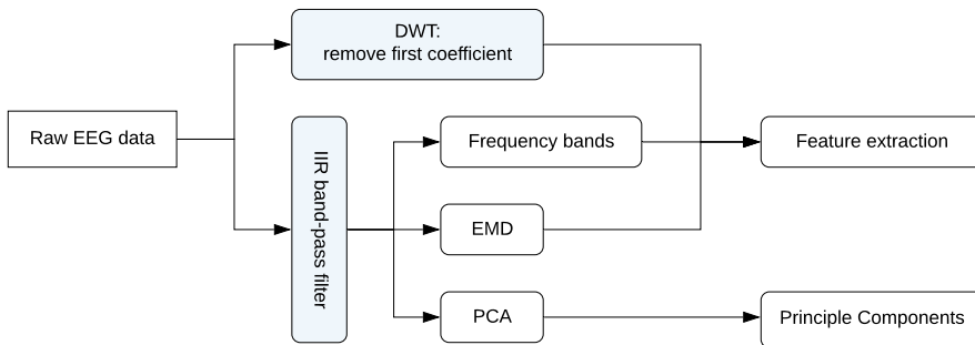
Figure 4.5: Pre-processing steps used on each dataset. For Dataset 1, IIR band-pass filter 1.0 - 20.0\text{ Hz} was applied, and for Dataset 2 an IIR band-pass filter 0.5 - 40\text{ Hz} .
