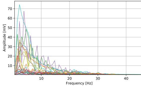
Figure A.2: Frequency spectrum of pre-processed resting-state data from Dataset 1.
